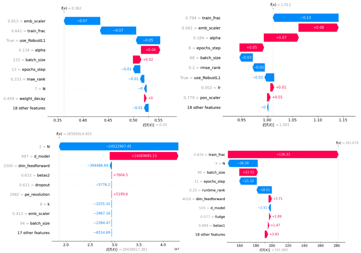
Figure 6. Waterfall SHAP analyses of Histogram Gradient Boosted Regressors trained on each of the different outputs. In clockwise order starting in the top left, MAE, RMSE, runtime, and model size.
